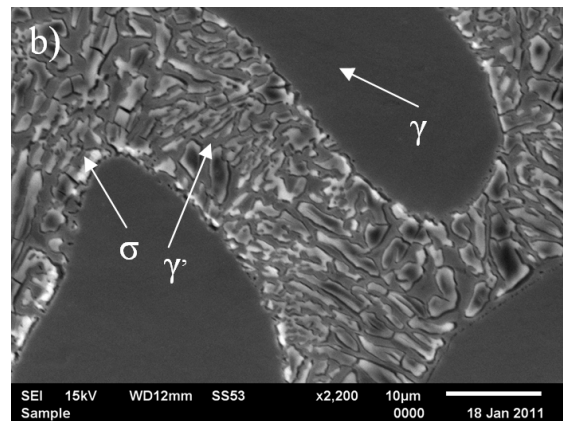
Fig. 2. Microstructures of cast steel: a) GX2CrNiMoCuN25-6-3-3 – solution heat treatment, b) GX2CrNiMoCuN25-6-3-1120°C/2h/water+800°C/3h, SEM
