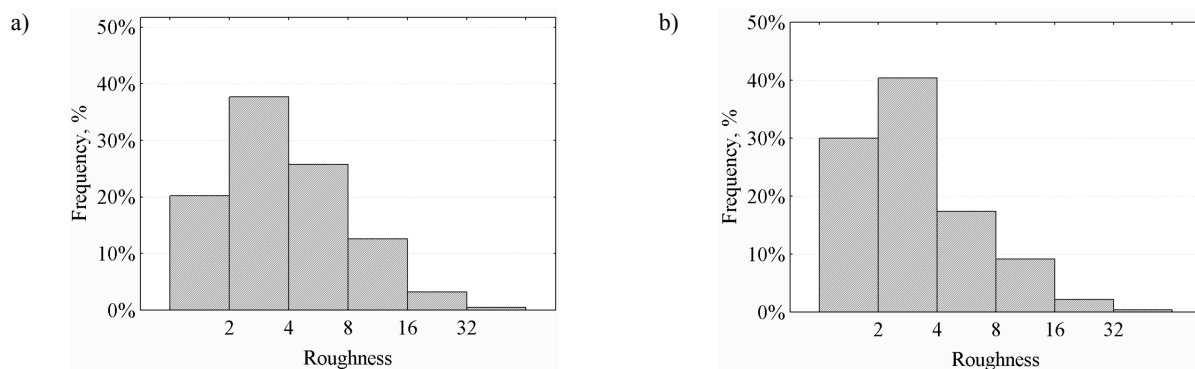
Fig. 5. Distribution of the shape factor R of the \sigma phase precipitates in cast steel with Cu addition annealed at the temperature of: a) 800°C, b) 900°C
