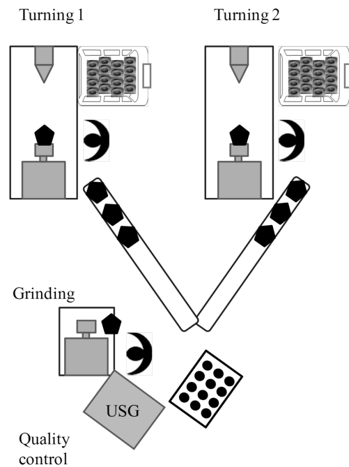
Fig. 6. Design of a machining cell
