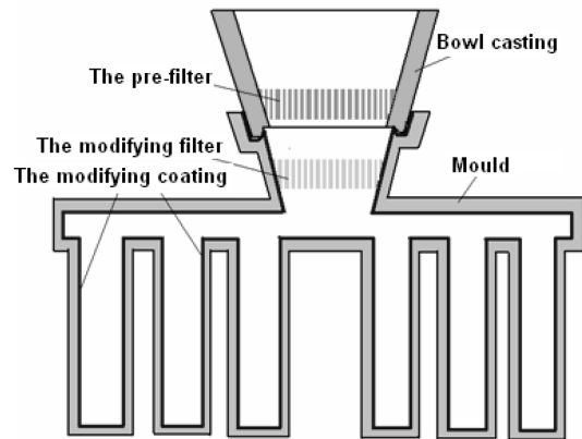
Fig. 1. Schematic diagram of the ceramic mould –filters location
