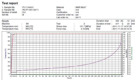
Fig. 10. Plotted results of creep test for MAR-247 (W) (white mould, blue filter) – time-related creep rupture strength (317 h 23 min.)
