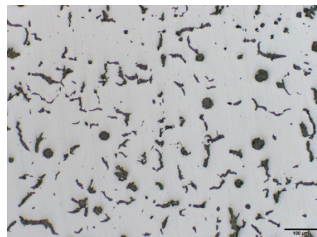
Wall thickness 16mm, 0.013%Mg, 15.2%SGI
