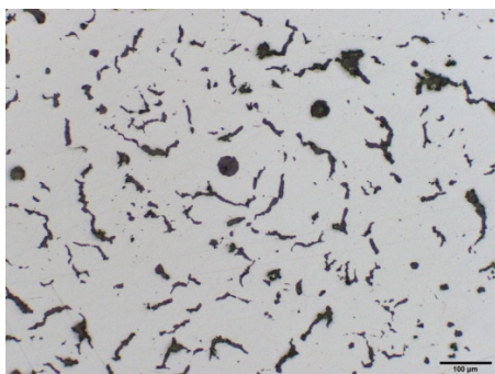
Wall thickness 20mm, 0.014%Mg, 9.35%SGI
