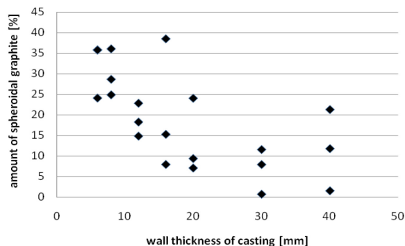
Fig. 3. Amount of spheroidal graphite depending on wall thickness of casting
