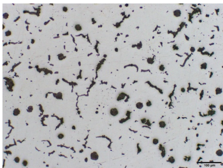
Wall thickness 12mm, 0.012%Mg, 14.8%SGI
