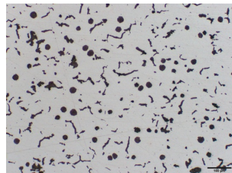
Wall thickness 8mm, 0.013%Mg, 24.9%SGI
