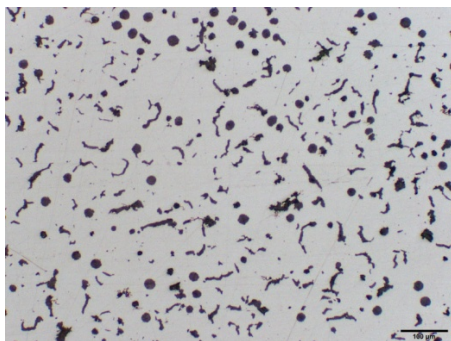
Wall thickness 6mm, 0.01%Mg, 35.8%SGI
