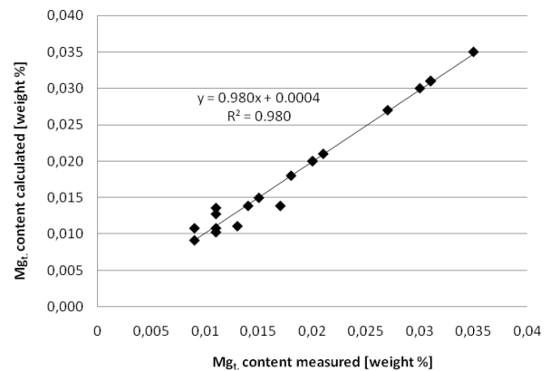
Fig. 1. Comparison of measured Mg content with calculated Mg content in t time
