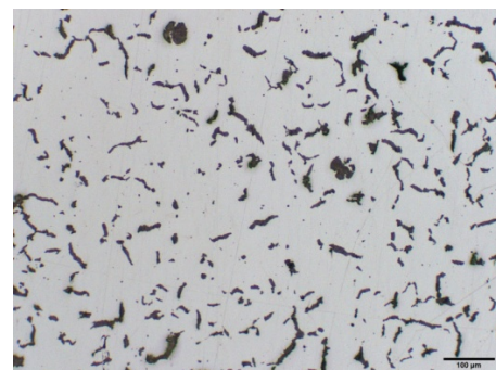
Wall thickness 40mm, 0.013%Mg, 1.5%SGI
