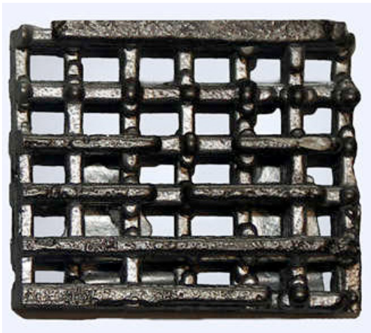
Fig. 3. Application of two stage investment casting for production of casting with regular cellular structure (obtained porosity 60-68%) at the Department of metallurgy and foundry VSB-TU Ostrava [5]
