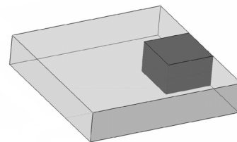
Sample 2: casting dimensions 100x100x20 mm, Mo=0,625cm
