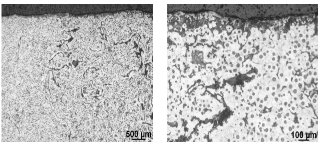
Fig. 4. Light photograph of the microstructure Sample 3 at different magnification
