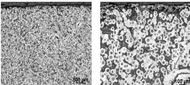
Fig. 3. Light photograph of the microstructure Sample 2 at different magnification
