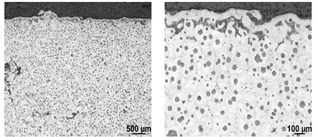
Fig. 5. Light photograph of the microstructure Sample 4 at different magnification
