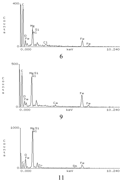
Fig. 7. Scanning photograph of the constituent in the structure of the casting Sample 4 with marked points, in which EDS analysis was performed. Below chosen spectrograms
