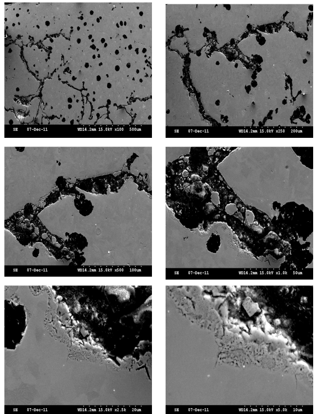
Fig. 6. Scanning photographs of the casting Sample 3, constituents in the structure at different magnification
