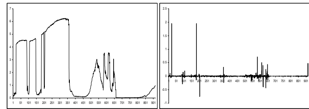
Fig. 3. Graphs of \text{CO}_2 concentration (testing set) and the error made by the model obtained by combined k -nn and M5 algorithms.
