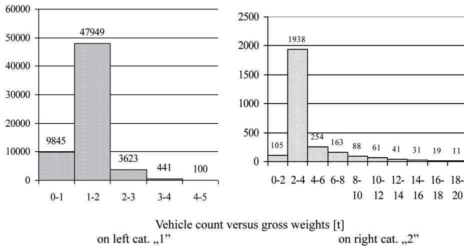
Fig. 7. Histograms of gross weights for vehicles passing through the point of measurement in days 1-9.12.2011 for lower categories
