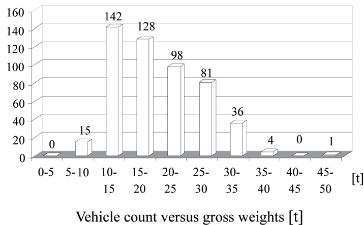
Fig. 8.a. Histograms of gross weights for vehicles passing through the point of measurement in days 1-9.12.2011 for category "3"
