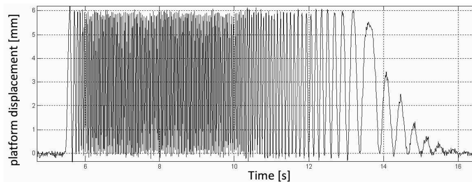
Fig. 4. Time history of platform vertical displacement during one full test according to UESAMA test procedure
