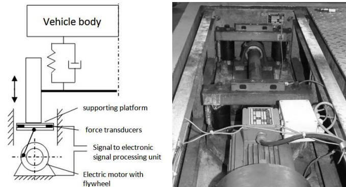
Fig. 3. Test bench working with EUSAMA principle: a) diagram, b) photography of partially disassembled test bench – from the bottom – view of electric motor, flywheel and shaft with a support bearing and with force transducers
