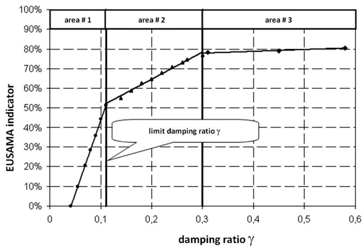
Fig. 6. Changes of EUSAMA indicator caused by damping ratio changes due to shock absorber wear [2]
