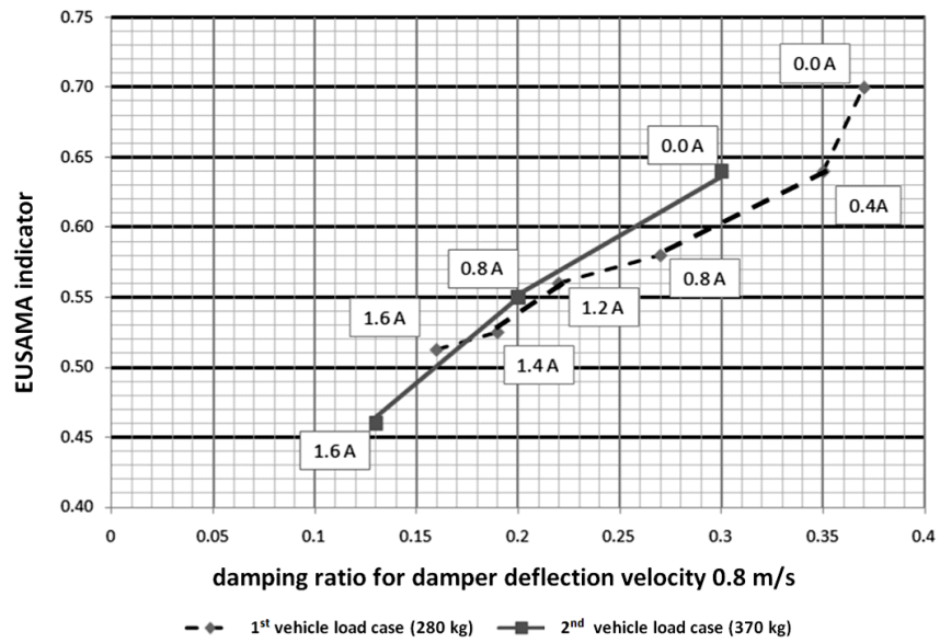
Fig. 5. Relation between damping ratio and EUSAMA indicator with variations of control current level and vehicle load
