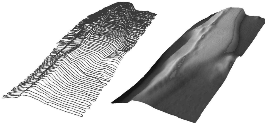
Fig. 3. Digital bottom model
