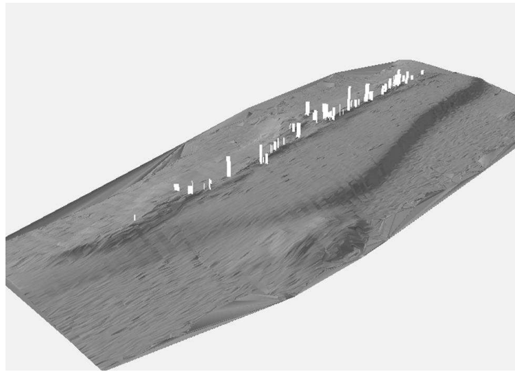
Fig. 6. Stones presented in the digital bottom model
