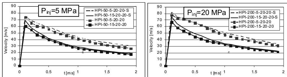
Fig. 8. Comparison of the results of the simulation (— lines) and the test stand investigations (--- lines) related to the influence of the backpressure and fuel injection pressure on the velocity of the front of the fuel spray ( P_{\text{inj}} = 5; 20 \text{ MPa} ; t_{\text{inj}} = 500 \text{ us} ; backpressure P_{\text{air}} = 0,5; 1,5 \text{ MPa} )
