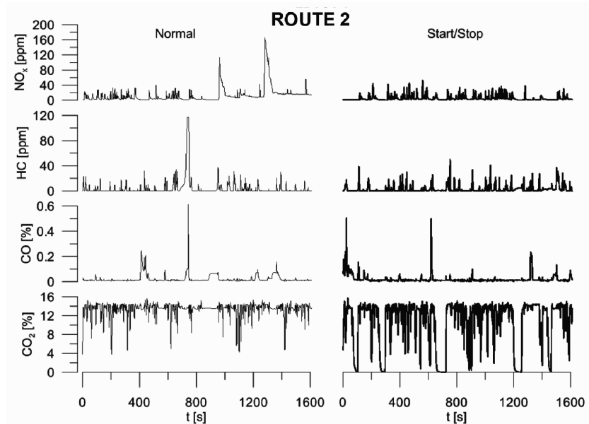
Fig. 6. Concentration of the exhaust emissions on route 2 (strict city center)
