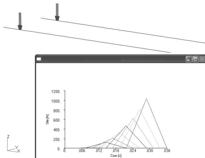
Fig. 5. The method of loading the model by example of few nodes
