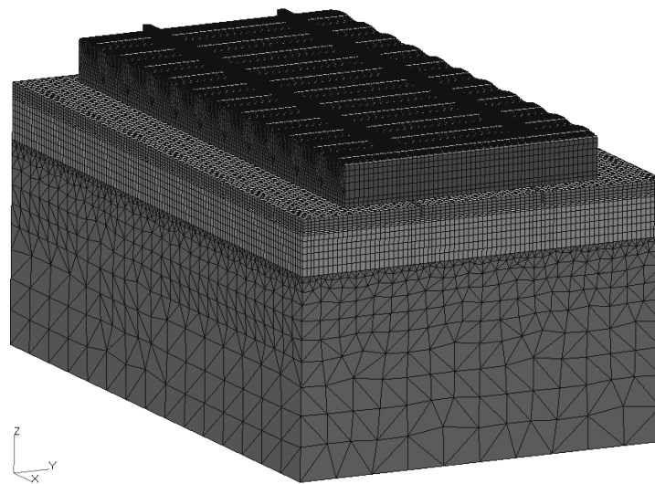
Fig. 3. Finite Element Model of the vibroinsulated trackage
