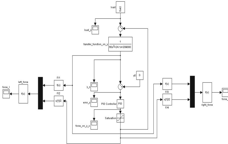
Fig. 13. The block diagram of the analysed control system modelled in the Matlab-Simulink environment
