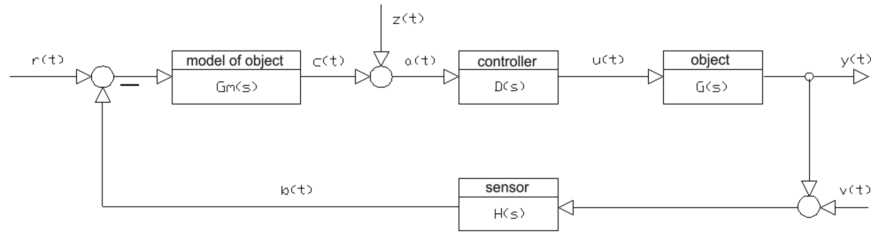
Fig. 12. The block diagram of the analysed control system with single feedback loop
