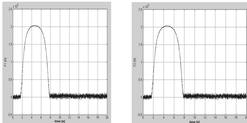
Fig. 15. a) and b) Time series of forces F_1 and F_2 in actuators 1 and 2 – y(t)
