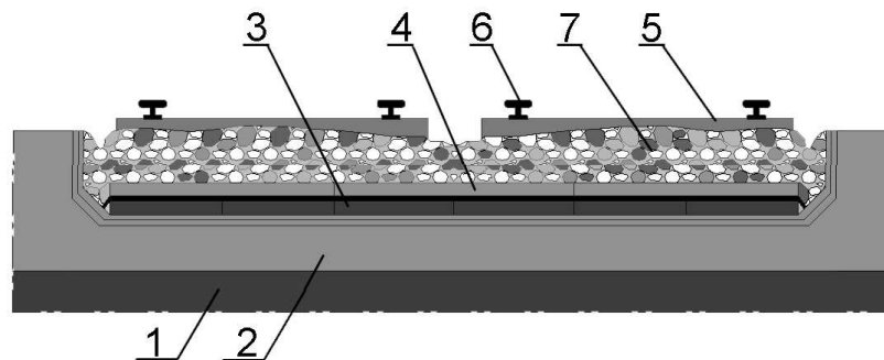
Fig. 1. The track on the vibroinsulating system (platform or viaduct version)
