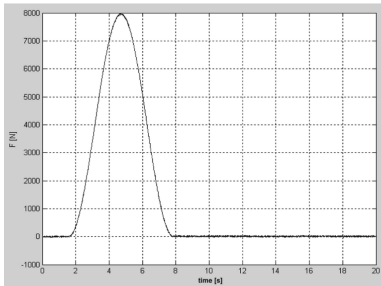
Fig. 14. Time series of the force F - u(t)
