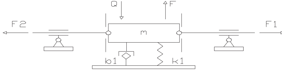
Fig. 11. Diagram of the vibroinsulation system
