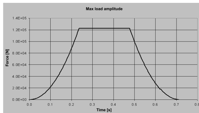
Fig. 6. Maximal amplitude of load as a function of time
