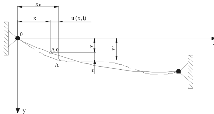
Fig. 10. Displacement of the point on the flexible tension member during the vibration in the plane of hanging
