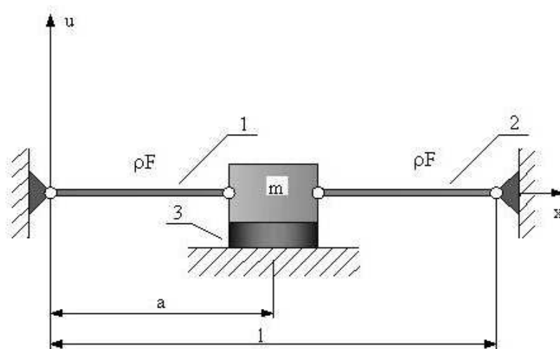
Fig. 9. The model of the vibroinsulation system for the railway crossing
