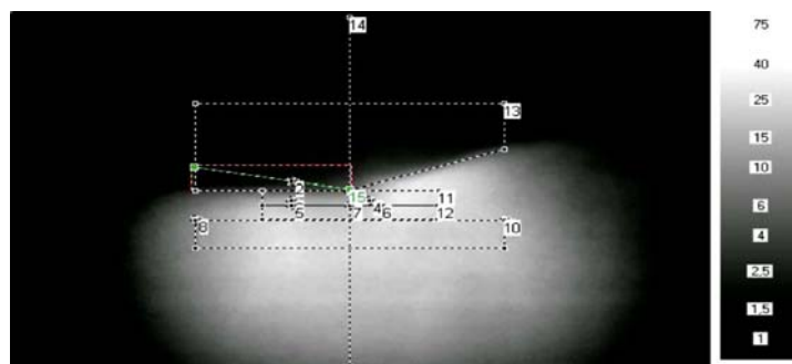
Fig. 8. The view of a light spot of low beam light reflector RE09237 (R2) together with indicated places of luminance measurement
