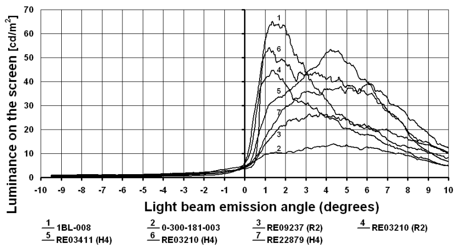
Fig. 32. Section within vertical axis V-V of light beam – borderline of light and shade
