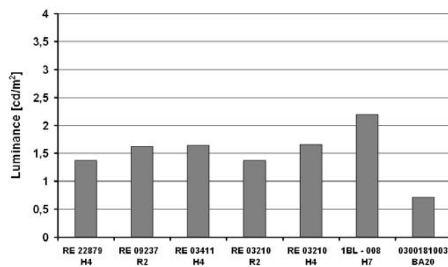
Fig. 30. Luminance values within Area 3 for the examined reflectors and projector
