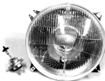
Fig. 13. Main light and low beam light reflector of RE03411 (029804) type with H4 light bulb
