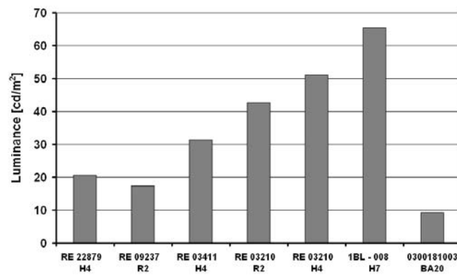
Fig. 23. Luminance values at the point 50V for the examined reflectors and projector
