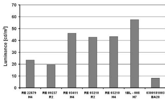
Fig. 25. Luminance values at the point 75R for the examined reflectors and projector
