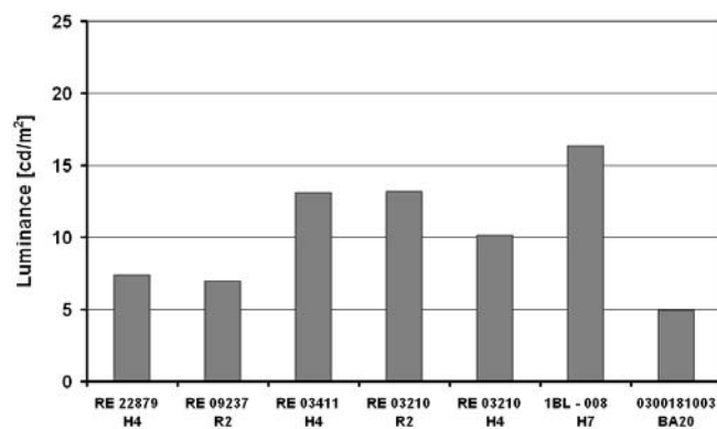
Fig. 26. Luminance values at the point HV for the examined reflectors and projector
