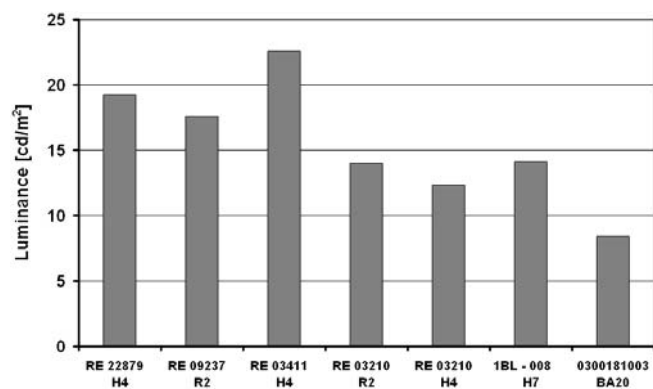
Fig. 20. Luminance values at the point 25R for the examined reflectors and projector
