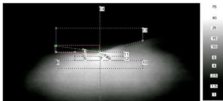
Fig. 10. The view of a light spot of low beam light reflector RE03210 (R2) together with indicated places of luminance measurement
