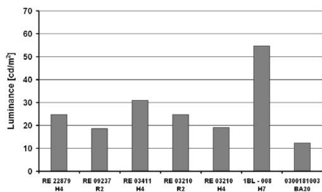
Fig. 21. Luminance values at the point 50L for the examined reflectors and projector
