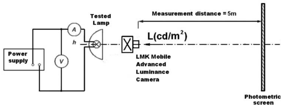
Fig. 2. Measurement station diagram
