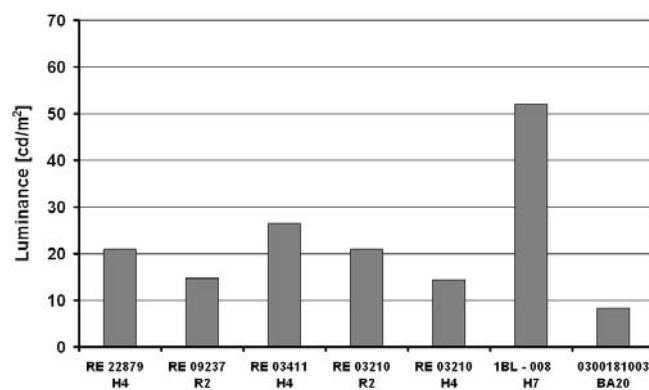
Fig. 24. Luminance values at the point 75L for the examined reflectors and projector
