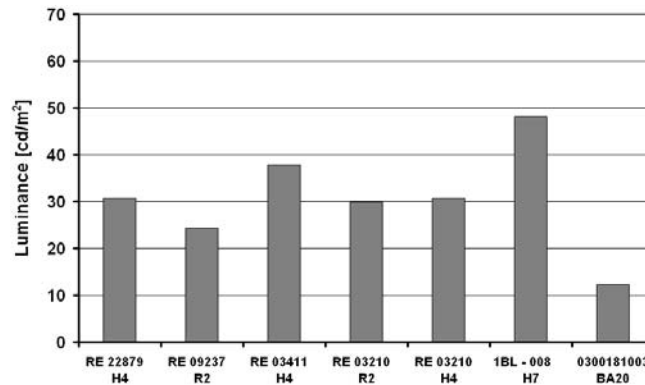
Fig. 31. Luminance values within Area 4 for the examined reflectors and projector
