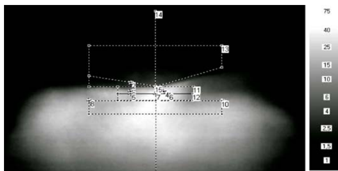
Fig. 16. The view of a light spot of main light reflector RE03210 (H4) together with indicated places of luminance measurement
