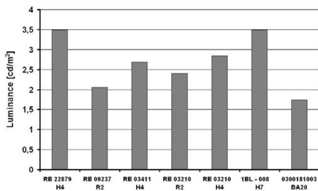
Fig. 27. Luminance values at the point B50L for the examined reflectors and projector
