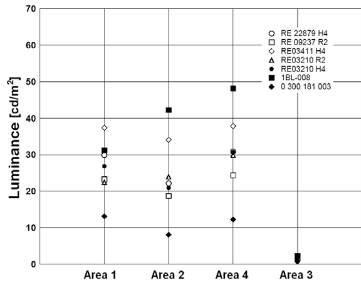
Fig. 18. Luminance measurement results in measurement areas of low beam light beams
