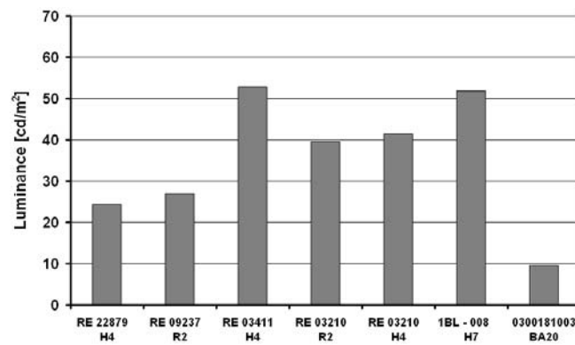
Fig. 22. Luminance values at the point 50R for the examined reflectors and projector
