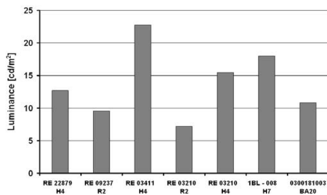
Fig. 19. Luminance values at the point 25L for the examined reflectors and projector
