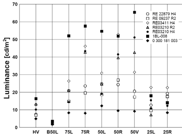
Fig. 17. Luminance measurement results in measurement points of low beam light beams
