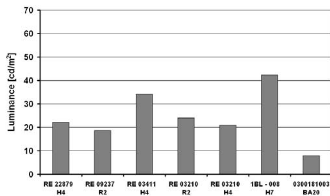
Fig. 29. Luminance values within Area 2 for the examined reflectors and projector
