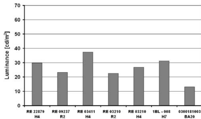
Fig. 28. Luminance values within Area 1 for the examined reflectors and projector
