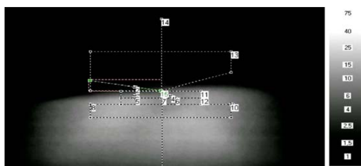
Fig. 5. Main light and low beam light reflector of 0-300-181-003 type with BA20D light bulb
