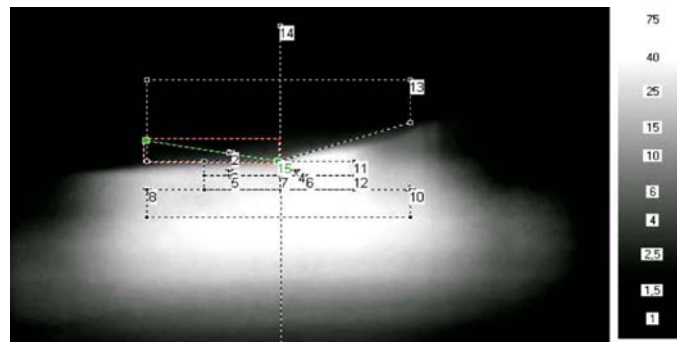
Fig. 14. The view of a light spot of low beam light reflector RE03411 (H4) together with indicated places of luminance measurement
