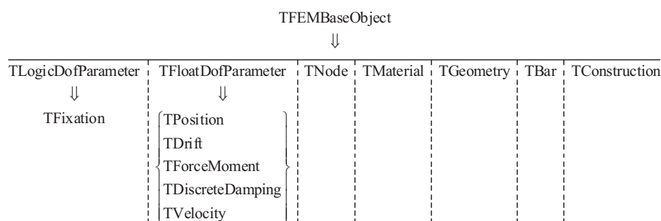
Fig. 3. FEM.pas topology of data classes
