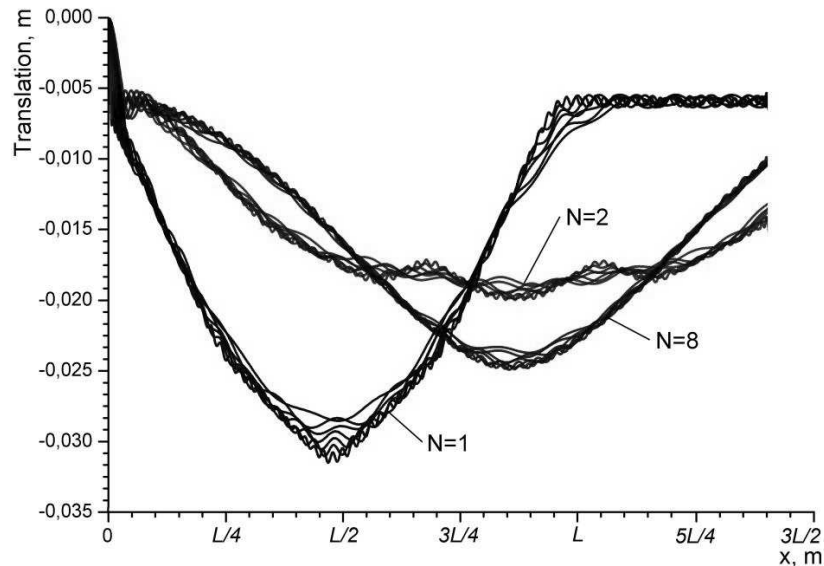
Fig. 7. Bending deflection of middle of span at different speeds of locomotive motion presented by the series of static forces, N quantity of forces
