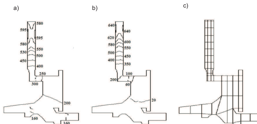
Fig. 9. Isothermal lines [°C] in the cross-section of front disc brake after: a) 15 repeated brake applications on the road (from v_1 = 100 km/h to v_2 = 50 km/h), b) braking on the Clayton roll-stand ( F_b = 1000 N, v_T = 62 km/h, t_b = 40 s), c) applied finite element mesh of brake disc and hub
