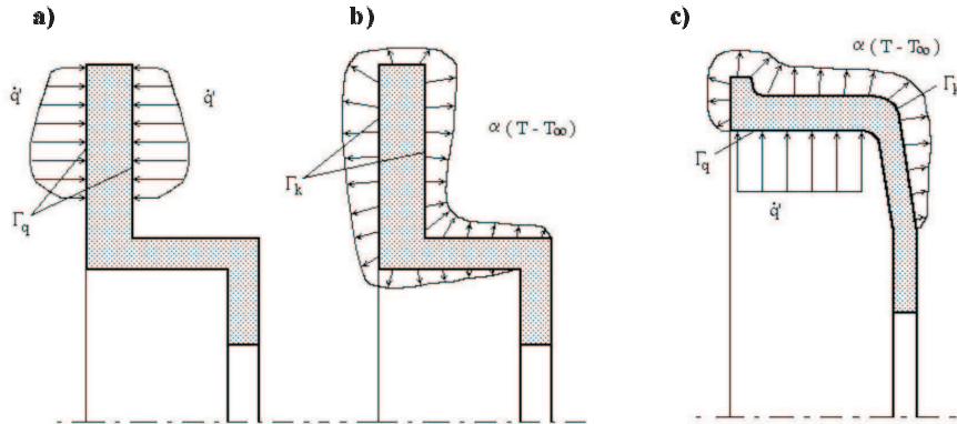
Fig. 1. Two-dimensional, axi-symmetrical model of unsteady heat transfer in brake rotors: a) heat flux q' generated on the friction surface \Gamma_q of disc brake, b) heat transferred to ambient air from free surfaces \Gamma_k of disc brake, c) boundary conditions of heat transfer in brake drum
