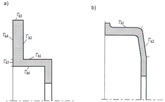
Fig. 2. Assumed surfaces of brake rotor concerning heat transfer to ambient air: a) disc brake ( \Gamma_{ki} , i=1, \dots, 6 ), b) drum brake ( \Gamma_{ki} , i=1, 2 )
