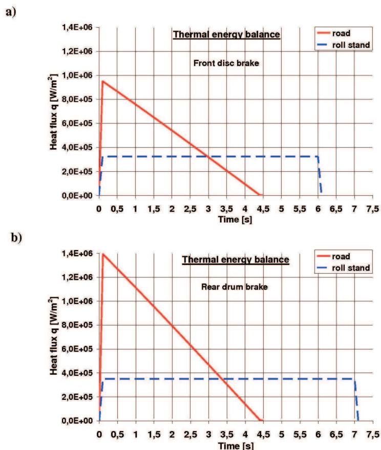
Fig. 3. Balance of thermal energy generated in car brakes during braking period. Braking on the road: initial velocity v_0 = 70 km/h, average deceleration a_b = 4,45 m/s 2 , braking time. t_b = 4,42 s. Braking on the Clayton roll-stand: test velocity v_T = 62 km/h, brake force F_b = 1000 N. Braking time on the roll-stand: a) t_b = 6 s for the front disc brake, b) t_b = 7 s for the rear drum brake
