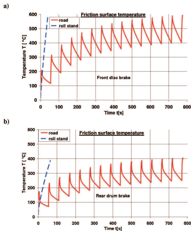
Fig. 8. Temperatures of the friction surfaces of car brakes during 15 repeated brake applications on the road (from v_1 = 100 km/h to v_2 = 50 km/h) and during constant braking on the Clayton roll-stand: test velocity v_T = 62 km/h, brake force F_b = 1000 N. Total braking time on the roll-stand: a) t_b = 40 s (for front disc brakes), b) t_b = 65 s (for rear drum brakes)
