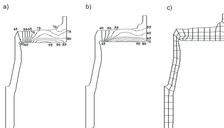
Fig. 6. Isothermal lines [ ^{\circ}\text{C} ] in the cross-sections of rear drum brake at the end of braking: a) on road from v_0 = 70 km/h, b) on the “Clayton” roll-stand ( F_b = 1000 N, v_T = 62 km/h, t_b = 7 s), c) applied finite element mesh of brake drum
