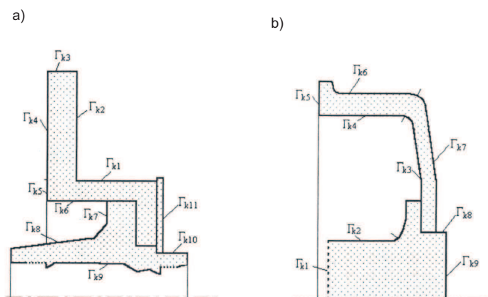
Fig. 7. Assumed surfaces of brake concerning heat transfer to ambient air in case of repeated brake applications: a) disc brake ( \Gamma_{ki} , i=1, \dots, 11 ), b) drum brake ( \Gamma_{ki} , i=1, \dots, 9 )
