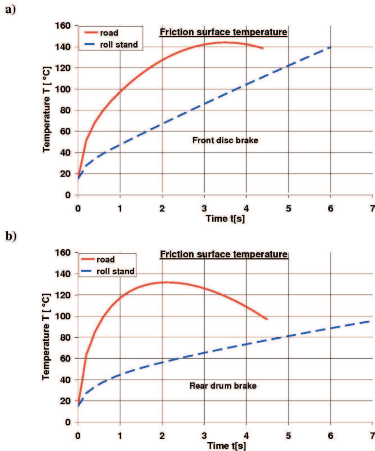
Fig. 4. Temperatures of the friction surfaces of car brakes versus time. Braking on the road: initial velocity v_0 = 70 km/h, average deceleration a_b = 4.45 m/s 2 , braking time t_b = 4.42 s. Braking on the Clayton roll-stand: test velocity v_T = 62 km/h, brake force F_b = 1000 N. Braking time on the roll-stand: a) t_b = 6 s (for the front disc brake), b) t_b = 7 s (for the rear drum brake)
