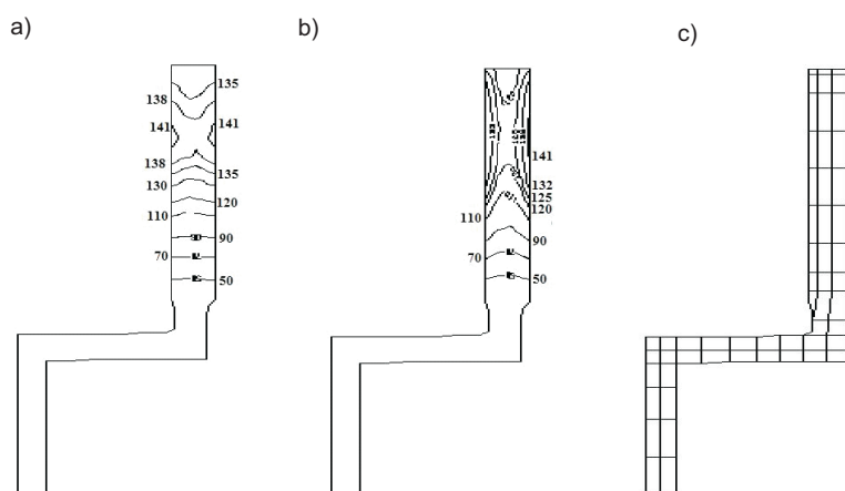
Fig. 5. Isothermal lines [ ^\circ\text{C} ] in the cross-sections of front disc brake at the end of braking: a) on road from v_0 = 70 km/h, b) on the Clayton roll-stand ( F_b = 1000 N, v_T = 62 km/h, t_b = 6 s), c) applied finite element mesh of brake disc
