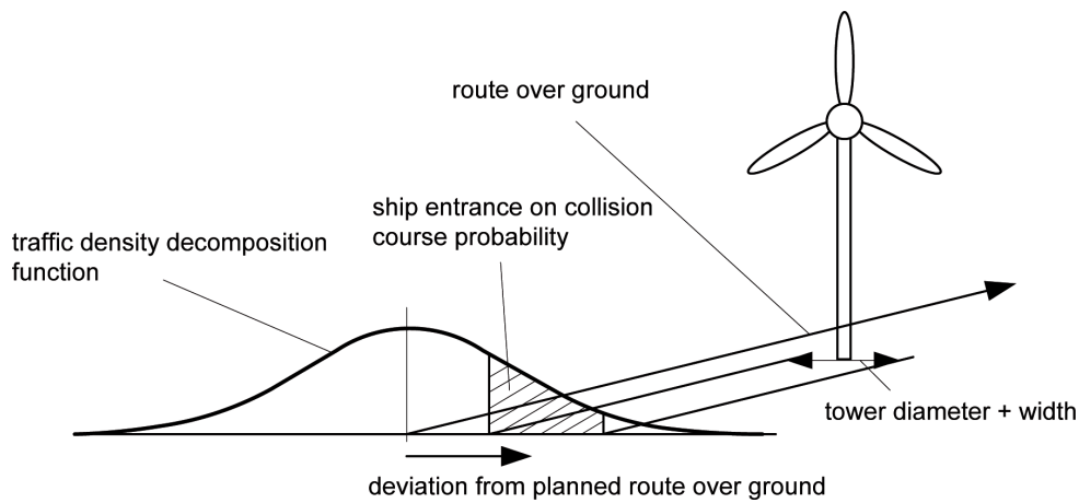
Fig. 1. Gaussian distribution of ships traffic density in direction perpendicular to the vectors of ships movement [4]
