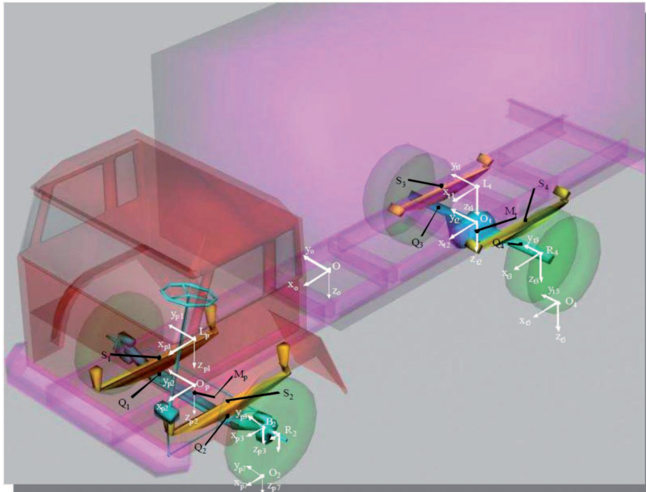
Fig. 1. General view of the truck model; characteristic points and coordinate systems
