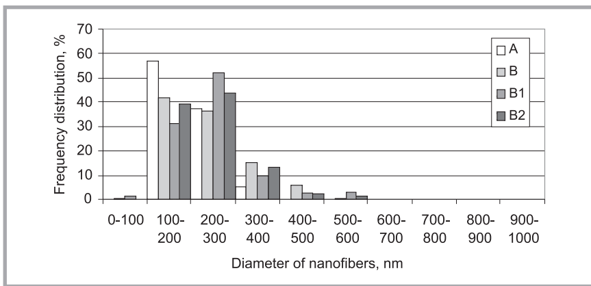
Figure 6. Frequency distribution of electrospun nanofibre diameter A - 100% PVA solution; B - 99% PVA with 1% amount of ethanol based 3 wt% iodine solution; B1 - 99% PVA with 1% amount of iodine based 6 wt% solution; B2 - 99% PVA with 1% amount of iodine based 9 wt% solution.
