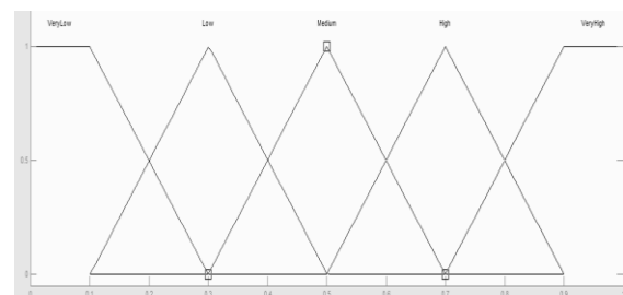
Figure 4. The membership function of the linguistics impact scale
