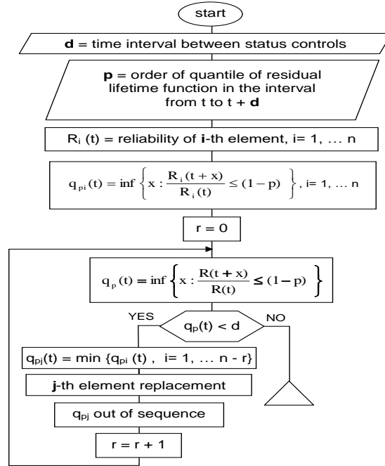
Fig. 2 Algorithm for selecting components for preventive replacement
