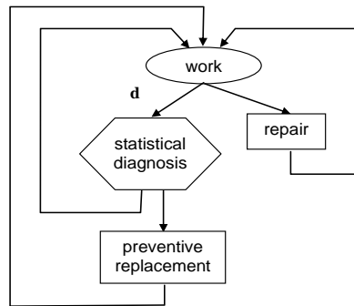
Fig. 3 Graph of model states (work – working of a system, statistical diagnosis – selecting a set of components, preventive replacement – replacement of selected components with new ones, repair – replacement of a failed component with a new one)
