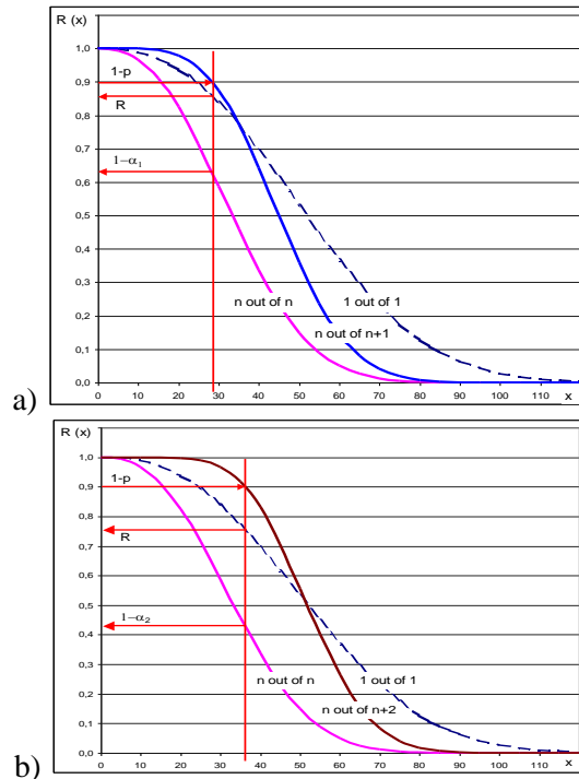
Fig. 1 Graphical interpretation of orders calculation on the basis of structures “n out of n+k”, “n out of n” and “1 out of 1”: a) “n out of n+1”, b) “n out of n+2”
