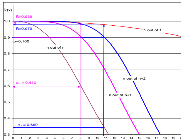
Fig. 4 Graphical interpretation of calculating new quantile orders
