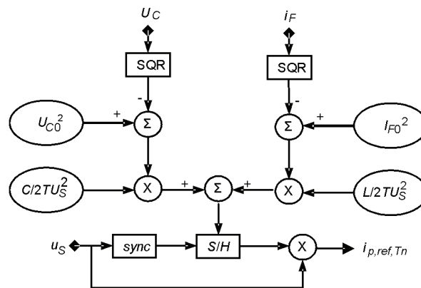
Fig. 6. The reference current obtaining scheme
