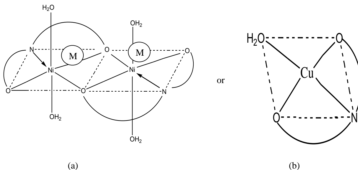
Figure 1. Structure of Schiff base complexes (a) M= Ni, Zn or Co, dimeric octahedral structure for Ni, Zn and Co complexes (b) Square planar structure for Cu complex
