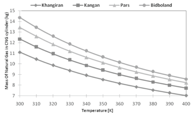
Figure 9. The effect of final in-cylinder temperature on mass of natural gas in CNG cylinder
