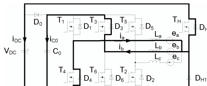
Fig. 7. Equivalent circuit of the converter during braking operation: T_1 is off
