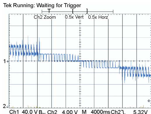
Fig. 8. The magnified view of the output waveform of the cascade inverter showing voltage modulation
