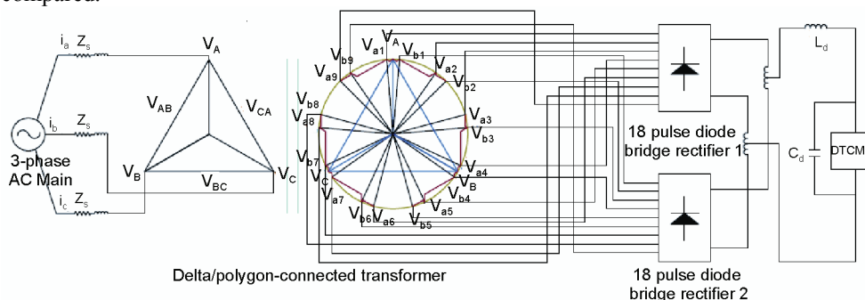
Fig. 1. Delta/polygon-transformer configuration for 36-pulse ac-dc conversion
