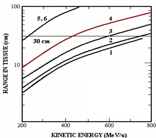
Fig. 3. Required ions kinetic energy for oncology therapy versus depth of penetration of beam for various nuclei:
