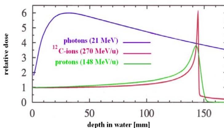
Fig. 1. Relative dose of irradiation versus depth inside water medium, for photons, protons and carbons ions
