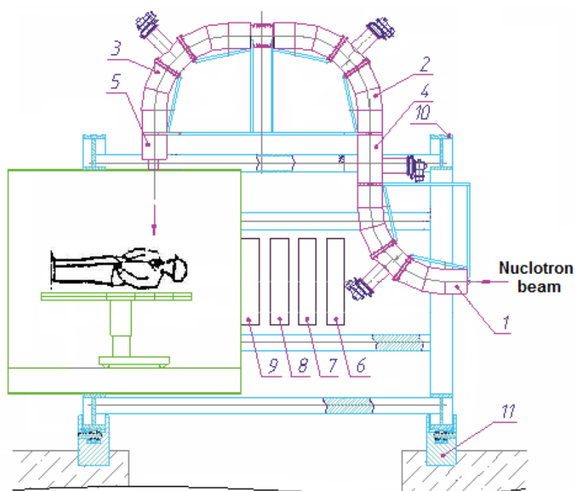
Fig. 5. Scheme of gantry project with superconducting magnets and cold heads cryocoolers: 1, 2, 3 – dipole magnets; 4 – focusing magnet; 5 – scanning magnet; 6 – sealing of helium tube; 7 – sealing of vacuum tube; 8 – electric siding connection; 9 – electric siding connection of cold head valves; 10 – frame of gantry; 11 – support of frame wheels
