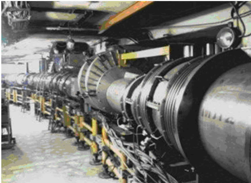
Fig. 4. View of the Nuclotron ring with superconducting electromagnets
