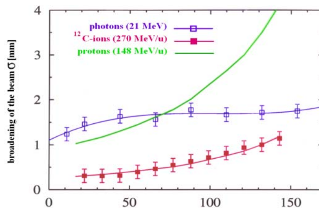
Fig. 2. Broadening of the irradiating beam versus depth inside water in mm for various kinds of irradiation
