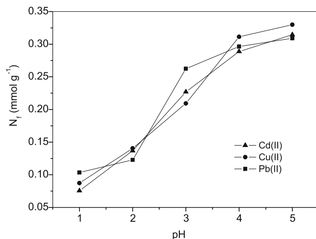
Figure 4. Influence of pH solution on the extraction process of Cu(II), Cd(II), and Pb(II). Experimental conditions: Temperature = 27^\circ\text{C} ; Si-BP mass = 0.05 g; Stirring time = 10 minutes
