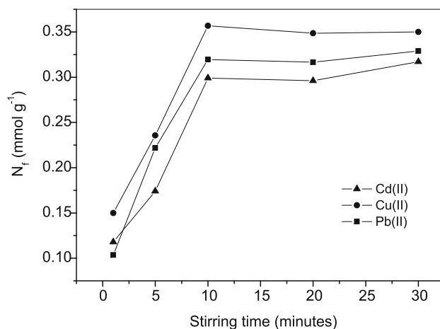
Figure 3. Dynamic equilibrium established by different stirring times in Cu(II), Cd(II), and Pb(II). Experimental conditions: Temperature = 27^\circ\text{C} ; Si-BP mass = 0.05 g; pH = 5.0.
