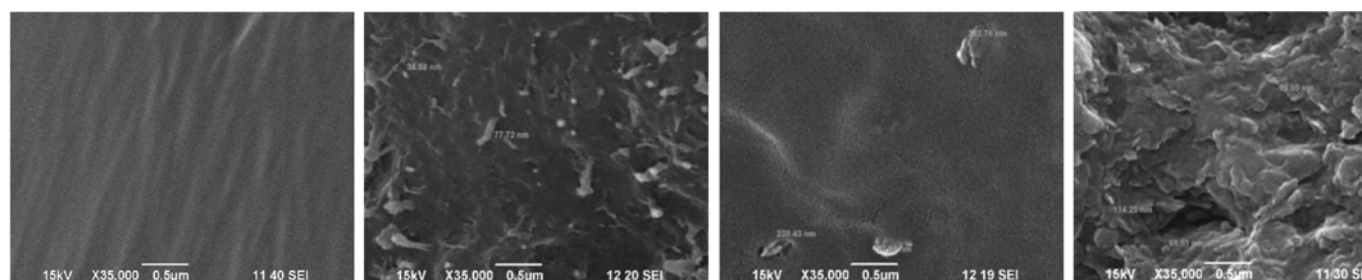
Figure 3. Microphotograph of SEM a) neat PP, b) PP_HNT unmod. , c) PP_HNT US , d) PP_HNT 450
