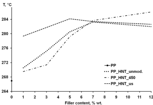
Figure 10. The influence of the content and HNT modification method on composites dropping point
