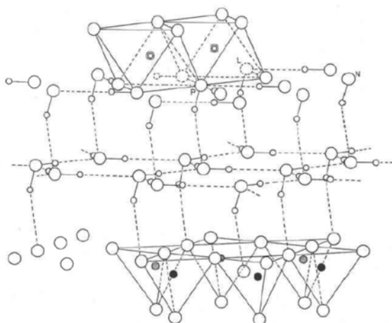
Figure 1. Hydrohalloysite structure 3
