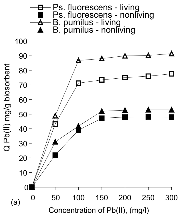
Figure 5. Effect of initial concentration of Pb(II) on their biosorption by living and nonliving cells. Incubation time 1h, temperature 30°C, pH 6.0
