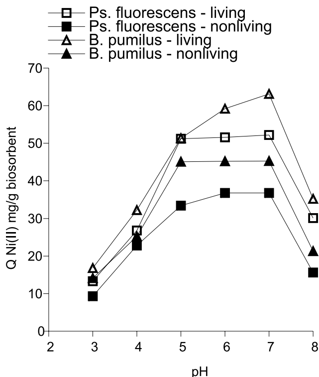
Figure 2. Effect of initial pH on biosorption capacity of Ni(II) by living and nonliving cells. Metal concentration 100 mg/l, temperature 30 ^{\circ}\text{C} , incubation time 1 h
