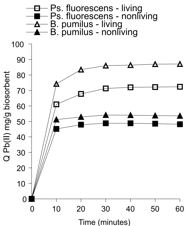
Figure 3. Effect of reaction time on biosorption capacity of Pb(II) by living and nonliving cells. Metal concentration 100 mg/l, temperature 30°C, pH 6.0
