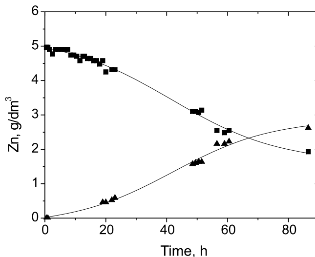
Figure 5. Change of zinc(II) concentration in time during membrane extraction-stripping process in the feed (■), and the stripping solution (▲) (Aqueous feed: 5 g/dm 3 Zn(II), 1.8% HCl, 5 M Cl - flow 0.25 cm 3 /s, Stripping solution: 1 M H 2 SO 4 , flow 0.25 cm 3 /s, PIM carrier: QPCI 20%)
