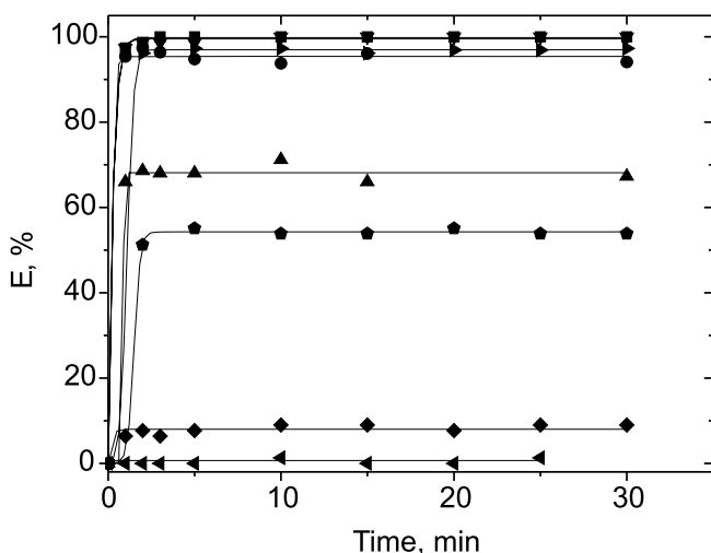
Figure 2. Extraction of Zn(II) vs. time with 0.2 M QPCL (■), QACL (●), QPBr (▼), QPNtf 2 (►), QABF 4 (▲), QPBF 4 (●), QPBis (◆), QPPF 4 (◄) (Aqueous feed: 5 g/dm 3 Zn(II), 1.8% HCl, 5 M Cl - )
