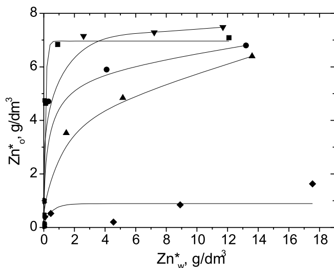
Figure 3. The isotherms of zinc(II) extraction with 0.2 M QPCL (■), QPBr (▼), QACL (●), QABF 4 (▲), QPPF 4 (◆) (Aqueous feed: 0.05 – 20 g/dm 3 Zn(II), 1.8% HCl, 5 M Cl - )
