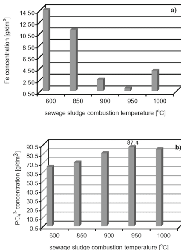
Figure 1. Influence of sewage sludge combustion temperature on Fe and \text{PO}_4^{3-} concentration in solutions after ash extraction with 3.68 mol/dm 3 \text{HNO}_3
