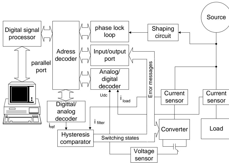
Fig. 2. Block scheme of a parallel active filter
