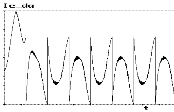
Fig. 6 Active filter reference current obtained using the p-q method
