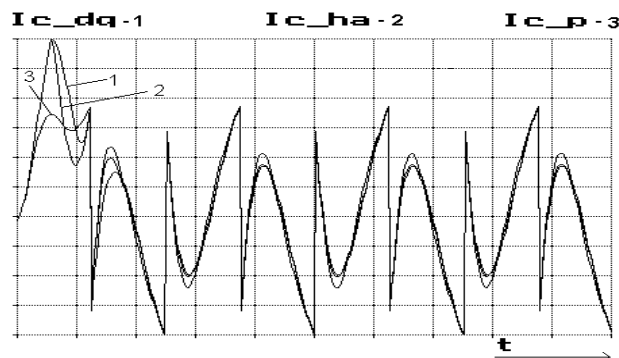
Fig. 5 Reference active filter currents computed by all three methods: 1 – p-q method; 2 – Fourier analysis method; 3 – moving average method
