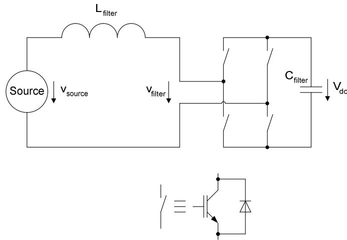
Fig. 3. Basic connection of a single-phase active filter
