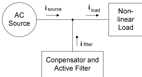
Fig. 1. Basic scheme of parallel compensation and filtering
