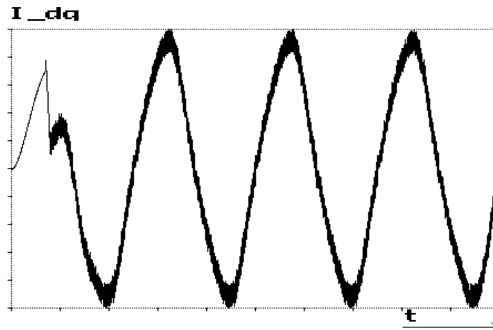
Fig. 7. Source current computed by the p-q method
