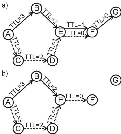
Fig. 3. The special case when a packet arrived earlier to the node E via nodes C and D: a) using EGQF protocol, b) using flooding protocol
