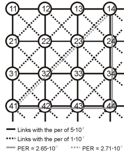
Fig. 1. An Example Fragment of the Sensor Network
