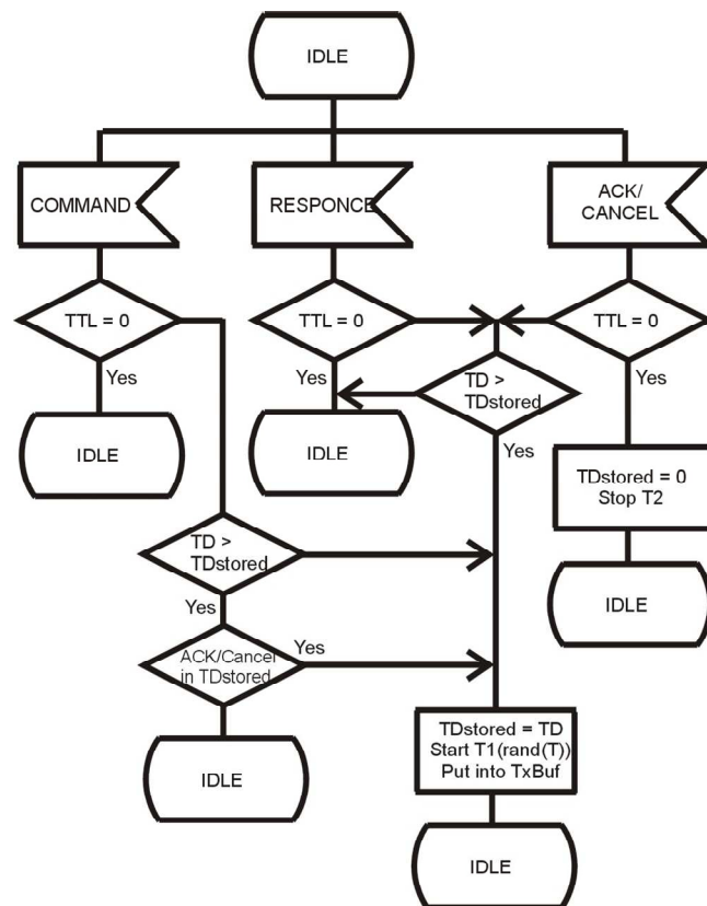
Fig. 2. A fragment of EGQF routing protocol algorithm
