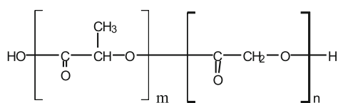
Poly(lactide-co-glycolide)
