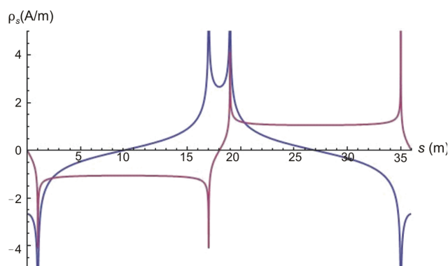
Fig. 8. Pole distribution for a rectangular region: aspect ratio 8 \times 1
