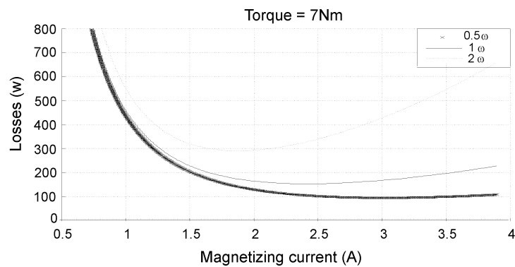
Fig. 5. Total loss versus magnetizing current at 7 Nms
