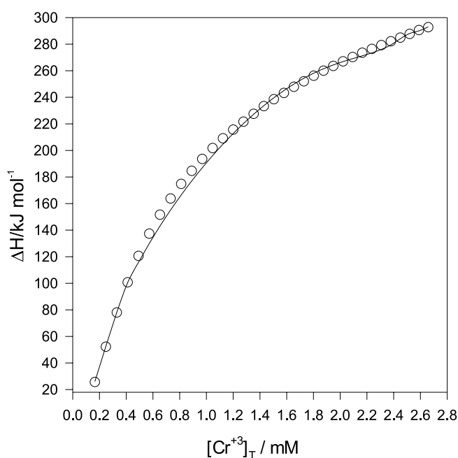
Figure 1. Comparison between the experimental enthalpies, ΔH, (O), for Cr 3+ +BLG-A interactions and calculated data (lines) via Eq. 6. [Cr 3+ ] T is the total concentration of Cr 3+ solutions in mM
