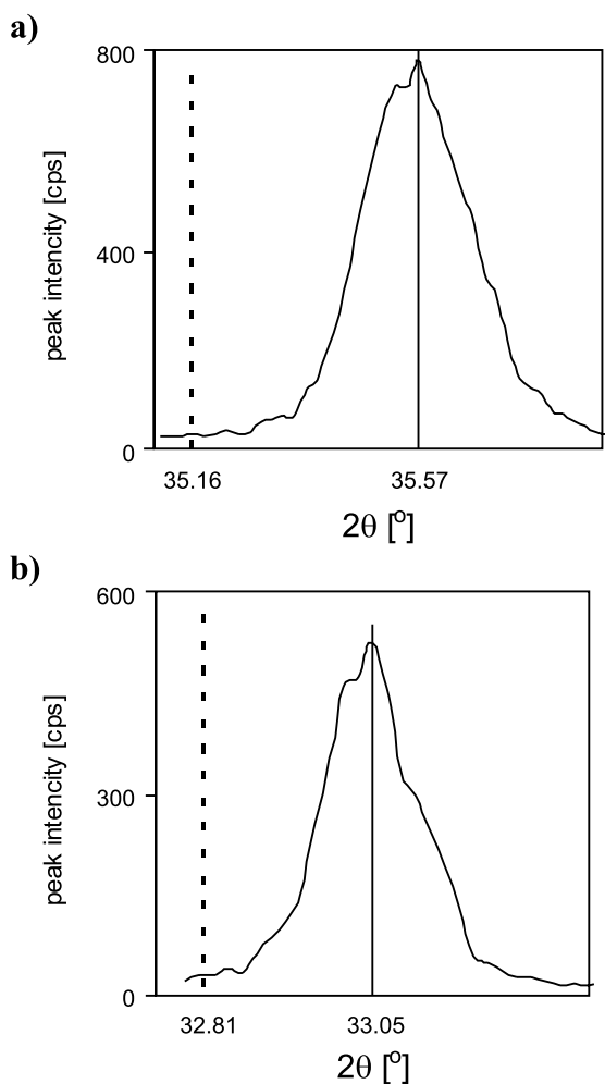
Figure 3. The most intense peak and corresponding standard pattern of: a) Ti-Co1 sample and Co 2 TiO 4 , b) Ti-Co4 sample and CoTiO 3
