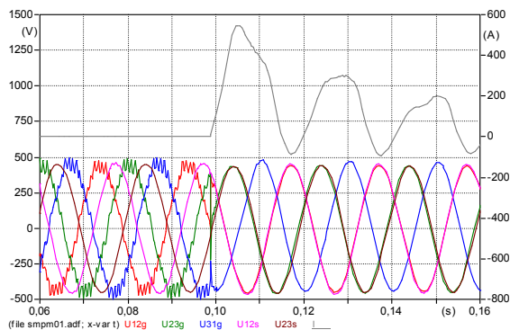
Fig. 8. The course of generator voltages ( U_{12g} , U_{23g} , U_{31g} (V)), voltages of distributive network ( U_{12s} , U_{23s} (V)) and course of current at the moment of generator connection to distributive network
