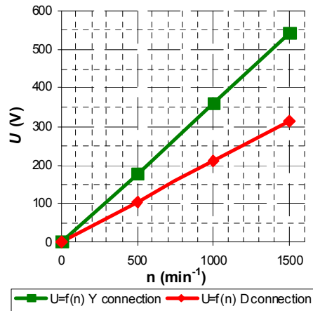
Fig. 5. The exciting characteristic of machine
