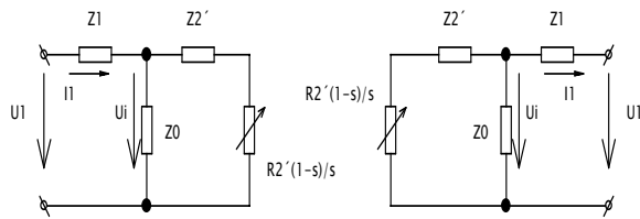
Fig. 1. The equivalent circuit of induction machine
