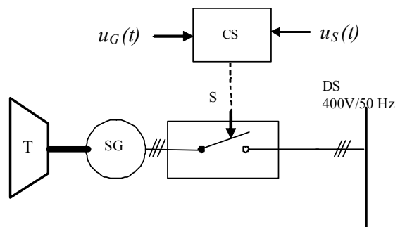
Fig. 6. The block scheme of control system of synchronous generator with permanent magnet.
