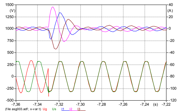
Fig. 2. Transient phenomena of switching induction generator to the distributive network
