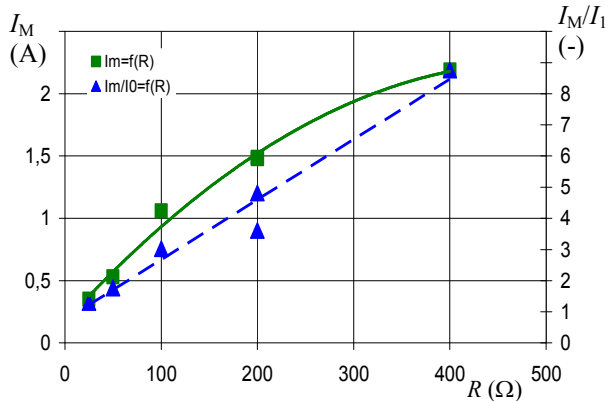
Fig. 3. The relation between over-current and size of resistor R
