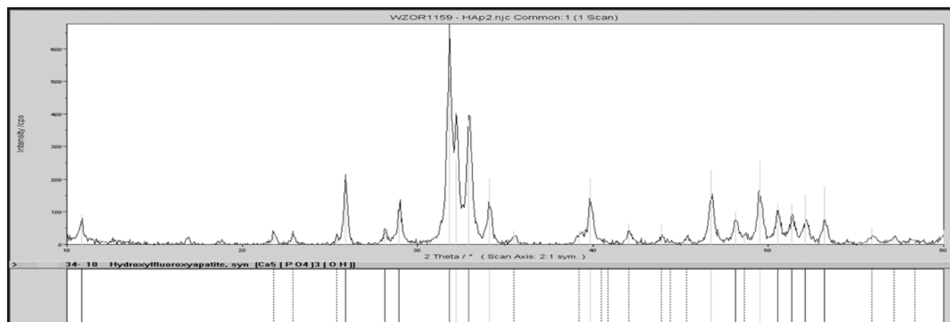
Figure 1. An X-Ray diagram of the calcining product obtained at the temperature of 650°C
