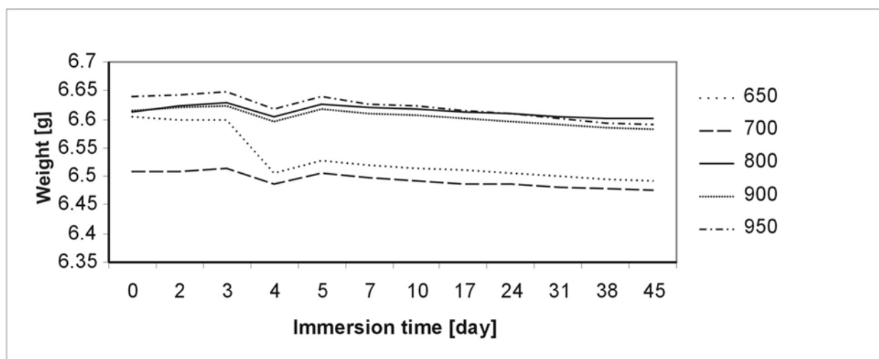
Figure 11. Changes in the mass of the samples immersed in distilled water
