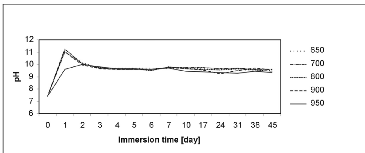
Figure 7. Changes in the pH value of distilled water
