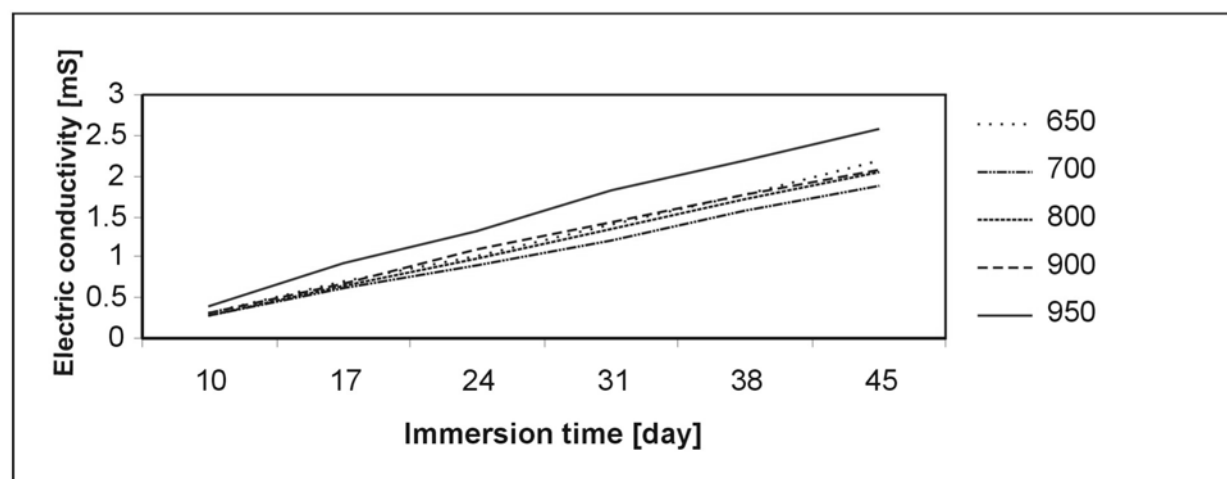
Figure 8. Changes in the electric conductivity of distilled water
