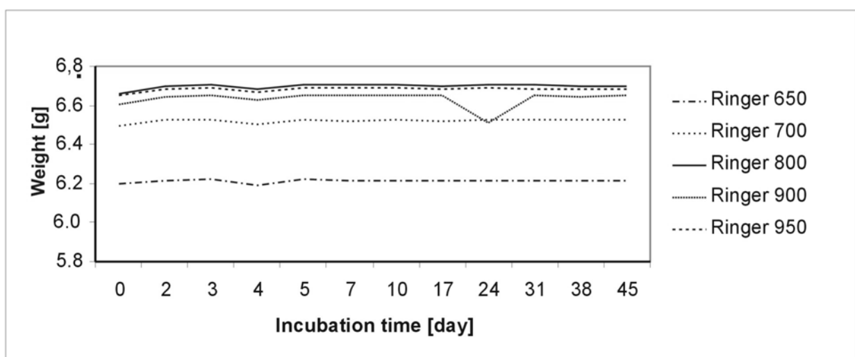
Figure 10. Changes in the mass of the samples immersed in Ringer liquid
