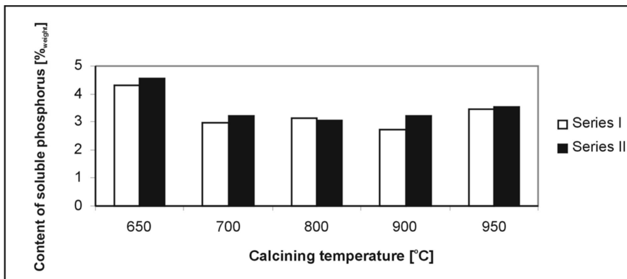
Figure 4. The content of phosphorus soluble in 2.0% citric acid in hydroxyapatite obtained at temperatures 650 – 950°C
