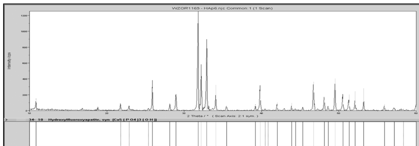
Figure 2. An X-Ray diagram of the calcining product obtained at the temperature of 950°C
