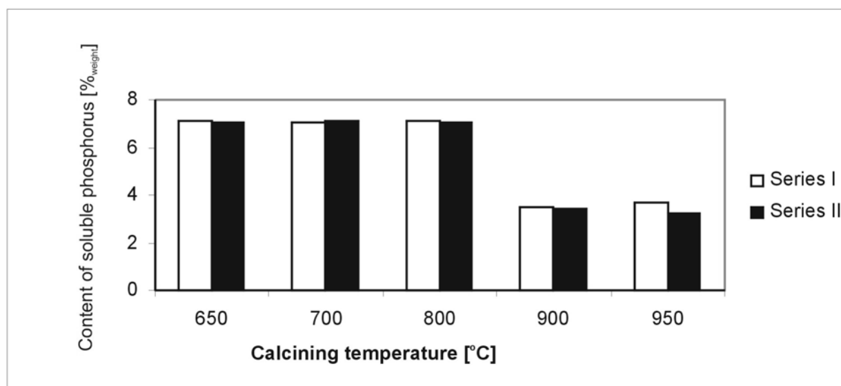
Figure 3. The content of phosphorus soluble in 0.4% hydrochloric acid in hydroxyapatite obtained at temperatures 650 – 950°C
