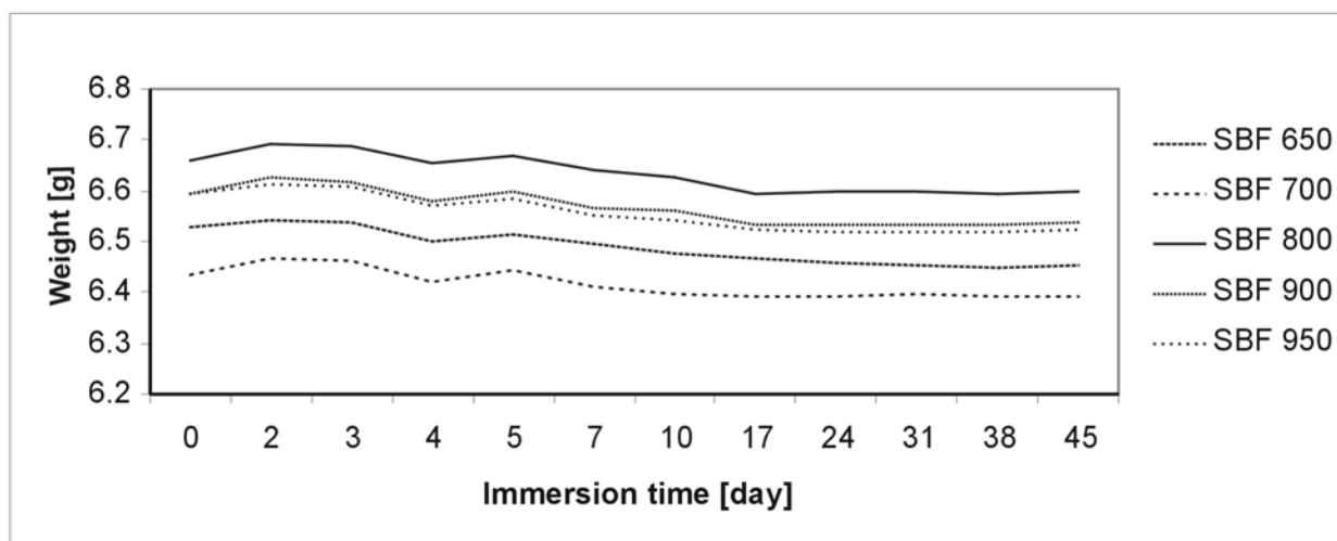
Figure 9. Changes in the mass of the samples immersed in SBF
