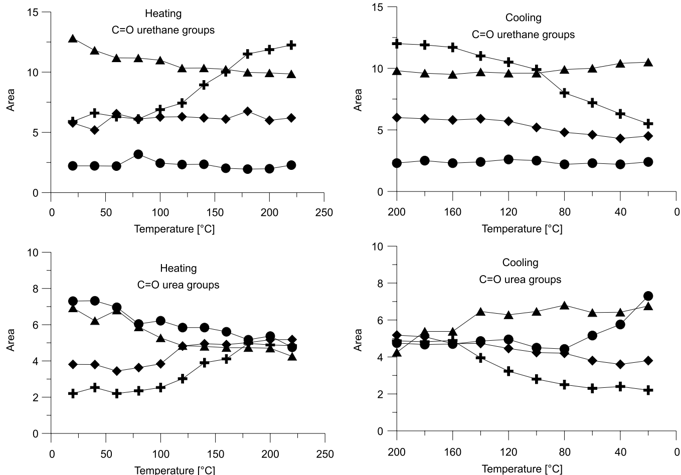
Figure 2. Changes in the areas of bands in amide I region during heating and cooling for PUU-650: + – free, ♦ – H-bonded disordered A, ● – H-bonded disordered B, ▲ – H-bonded ordered
