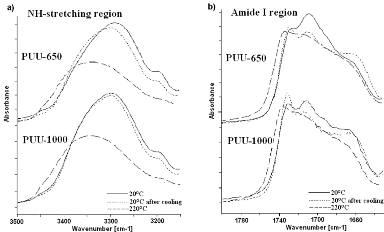
Figure 1. FTIR spectra of PUUs recorded at 20°C, 220°C and after cooling to 20°C
