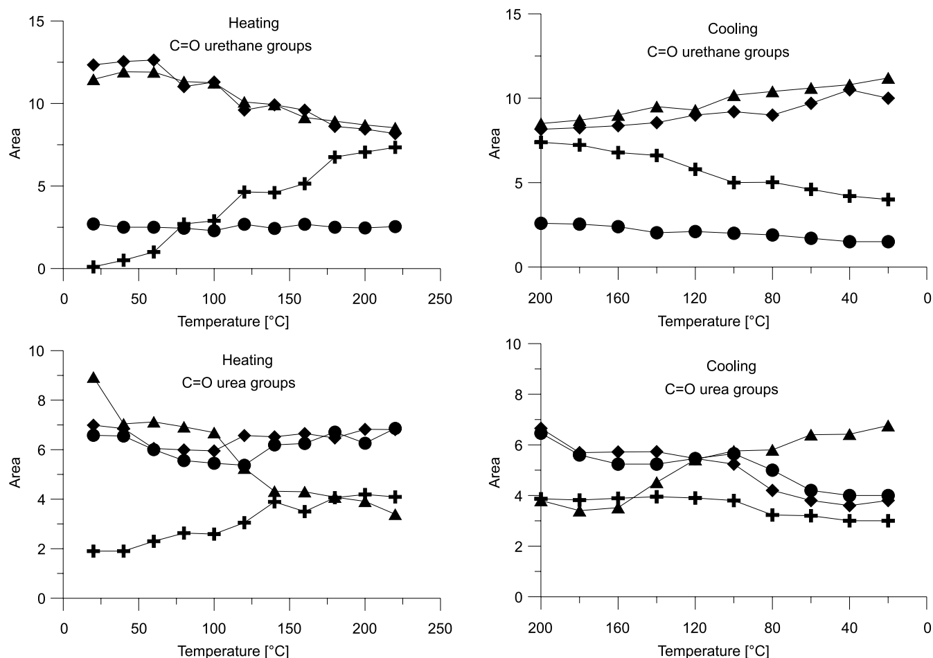
Figure 3. Changes in the areas of the bands in amide I region during heating and cooling for PUU-1000: + – free, ◆ – H-bonded disordered A, ● – H-bonded disordered B, ▲ – H-bonded ordered
