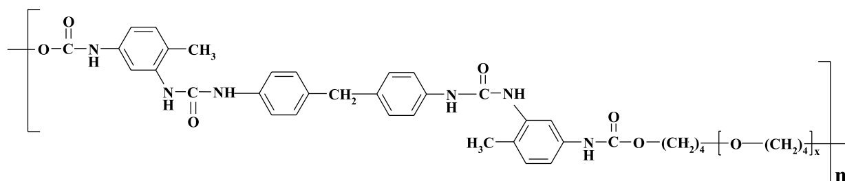
Scheme 1. Chemical structure of PUUs
