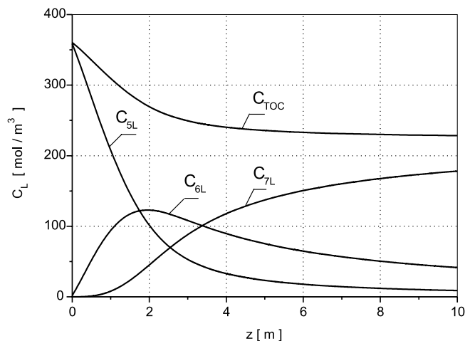
Figure 6. Composition profiles of S, T, K and global TOC in the bubble column 5 ≡ S, 6 ≡ T, 7 ≡ K
