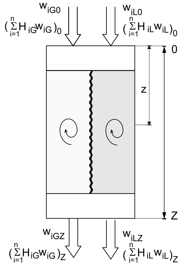
Figure 2. Schematic diagram of bubble columns
