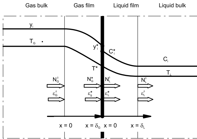
Figure 1. Scheme of mass and heat transfer
