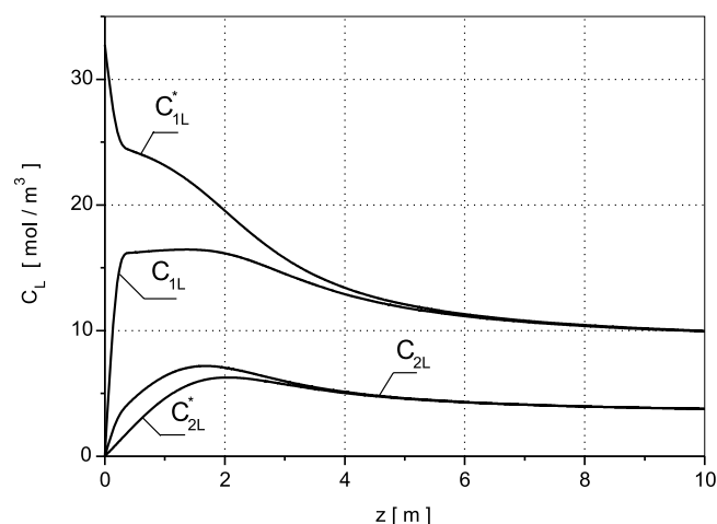
Figure 5. Composition profiles of O 2 and P(CO 2 ) in the bubble column 1 ≡ O 2 , 2 ≡ P (CO 2 )
