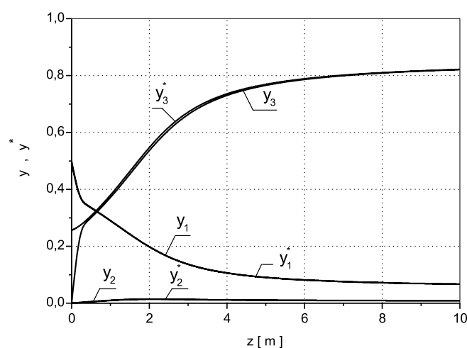
Figure 4. Composition profiles in the bubble column 1 ≡ O 2 , 2 ≡ P (CO 2 ), 3 ≡ H 2 O
