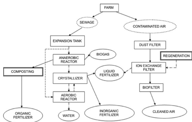
Fig. 3. Flow diagram of the integrated process of treating wastewater from animal farming [4]
