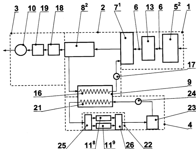
Fig. 2. Flow diagram of a plant for generating and processing thermal energy from liquid manure, agricultural waste and food processing waste [27]
