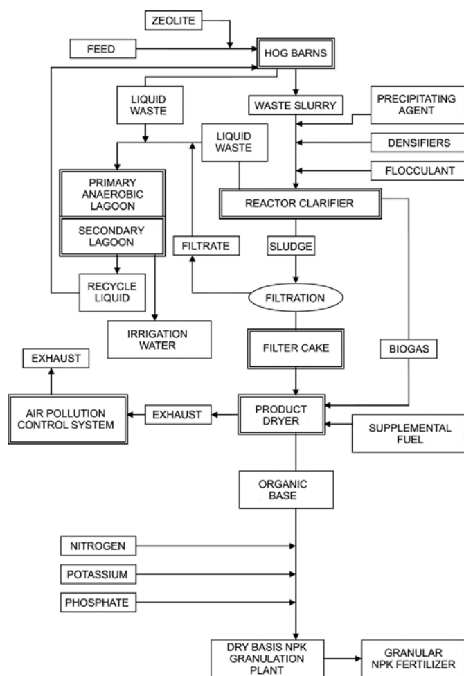
Fig. 1. Block diagram of pig manure processing methods [11]
