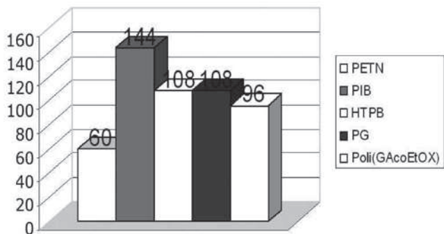
Fig. 2. Comparison of friction sensitivity of pure PETN and its mixtures
