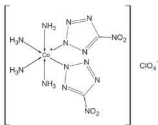
Fig. 3. Structure of BNCP
