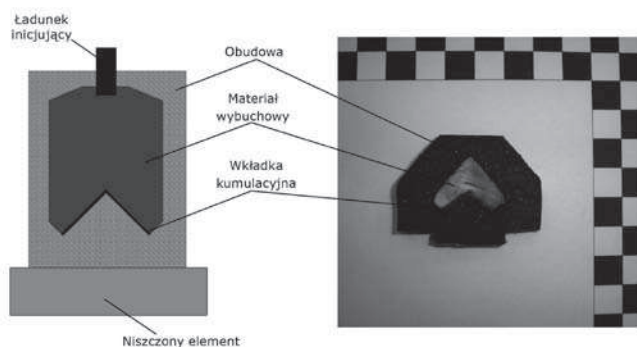
Fig. 4. Scheme of a flexible linear shaped charge (left) and a photo of a flexible linear shaped charge „BLADE” (right)
