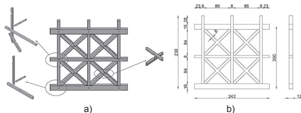
Fig. 2. Wall specimens: (a) connections used; (b) dimensions of elements in cm
