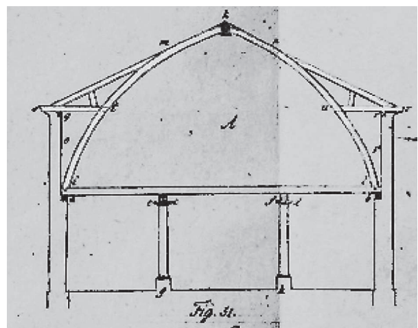
Fig. 9. recommended arched roof for storage buildings and packhouses. [11] Fig. 51
