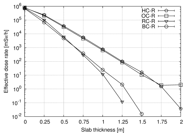
Fig. 9. Effective dose rate, calculated for human standing behind the slab. RUS concretes
