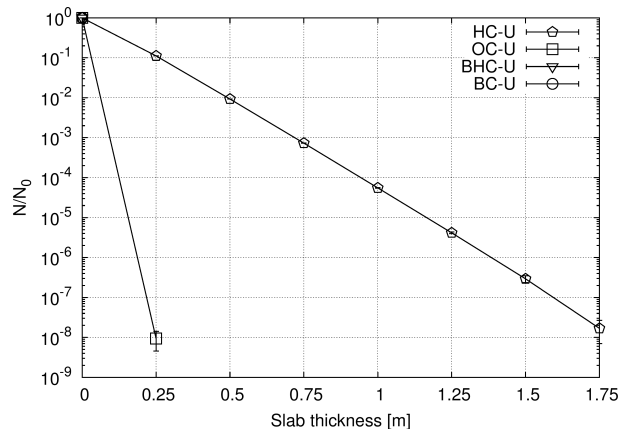
Fig. 18. Monoenergetic neutrons attenuation in Ulysse ordinary concrete
