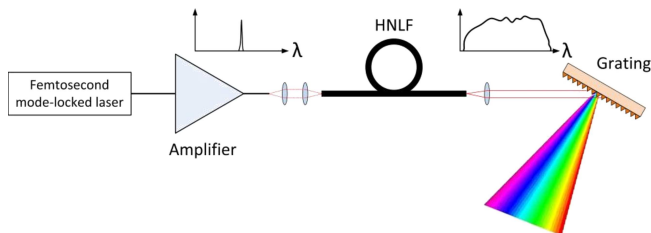
Fig. 11. Supercontinuum generation in HNLF
