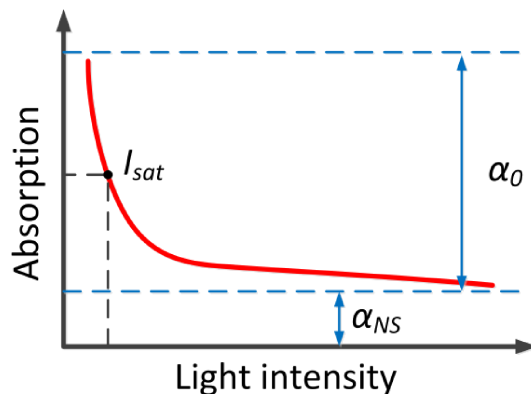
Fig. 4. Power-dependent absorption of a saturable absorber
