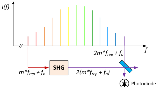
Fig. 10. The idea of a self-referencing frequency comb via f-2f interferometer
