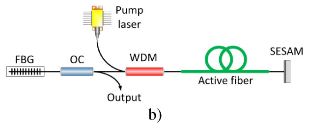
Fig. 7. A typical SESAM structure (a), typical fiber laser mode-locked by SESAM (b)
